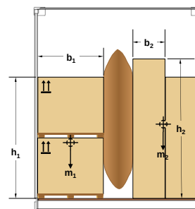
Figure 7.60 Unequal height packages
