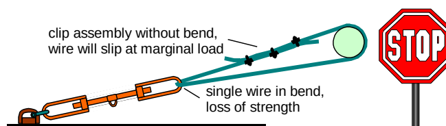
Figure 7.15 Improper assembly for wire rope lashing
