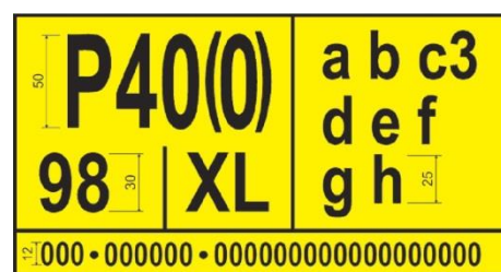
Figure 4.5 Yellow operational mark for trailers
