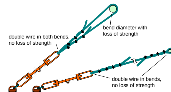
Figure 7.14 Recommended assemblies for wire rope lashing
