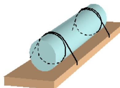
Figure 7.44 Silly-loop lashing
