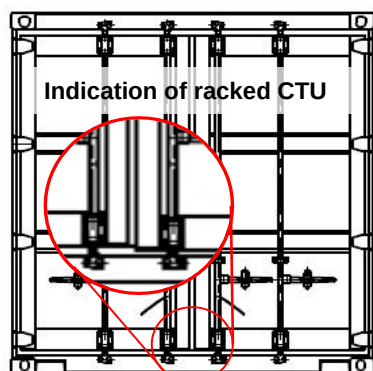
Figure 5.29 Racked CTU
