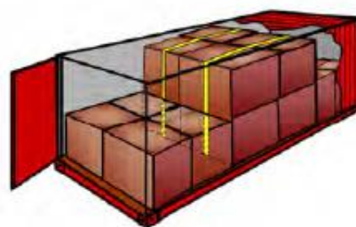
Figure 7.36 Round turn lashing
