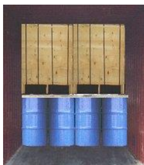
Figure 7.27 Mixed stow, dry over wet goods
