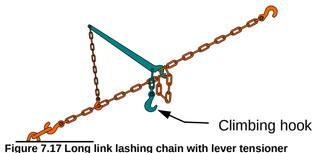
Figure 7.17 Long link lashing chain with lever tensioner
