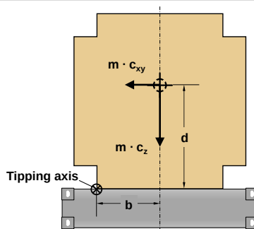
Figure 7.37 Tipping criterion
