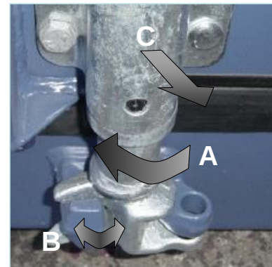
Figure 5.28 Door cam operation
