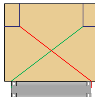
Figure 7.48 Transverse spring lashing
