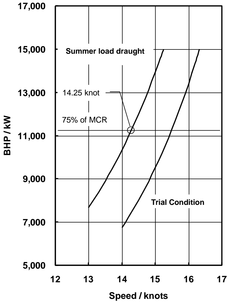
Figure 2.1: Power curves
